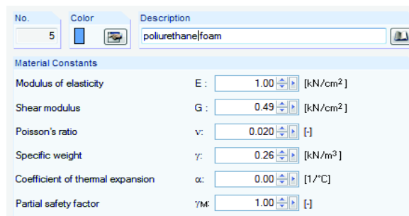
Figure 7. Polyurethane foam parameters
