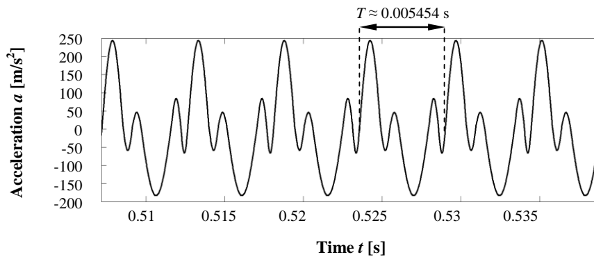
Figure 1. The signal curve of vibration accelerations at the handle modelled on the basis of recorded data, with the basic section indicated
