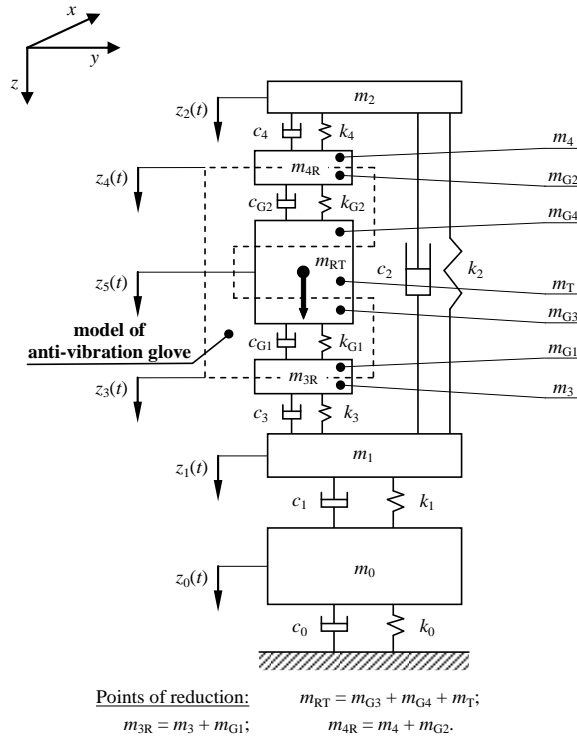
Figure 2. Physical model of the biodynamic H – G – T system created by combing the physical model of the human body and the glove model described in ISO 10068:2012 [9] with the tool model
