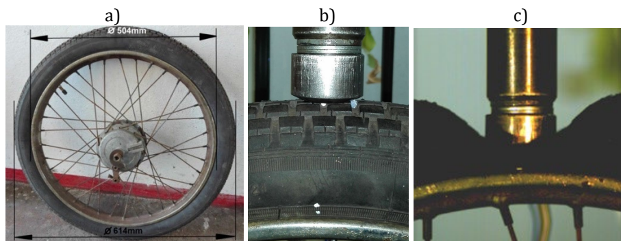
Figure 2. a) The wheel, b) the beater at the initial contact with the tyre tread, c) deformation of the tire under impact loading by means the beater.
