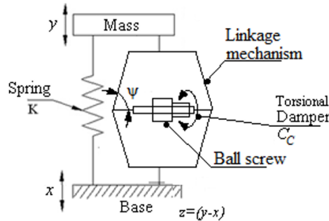
Figure 2. a): Ball screw based harvester without amplification, b): Ball screw based harvester with amplification, c): Ball screw based harvester with linkage mechanism for amplification.
